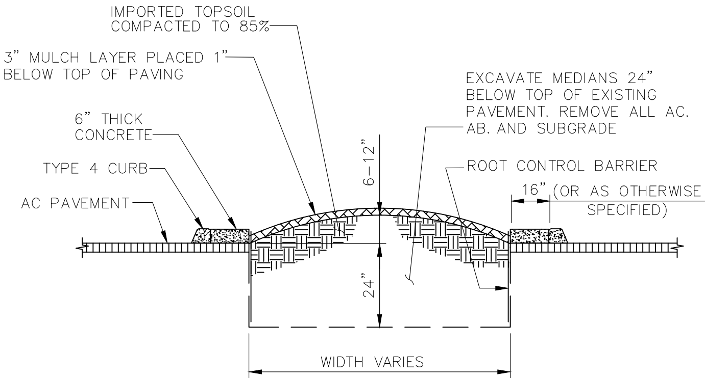
TYPE 4 CURB
