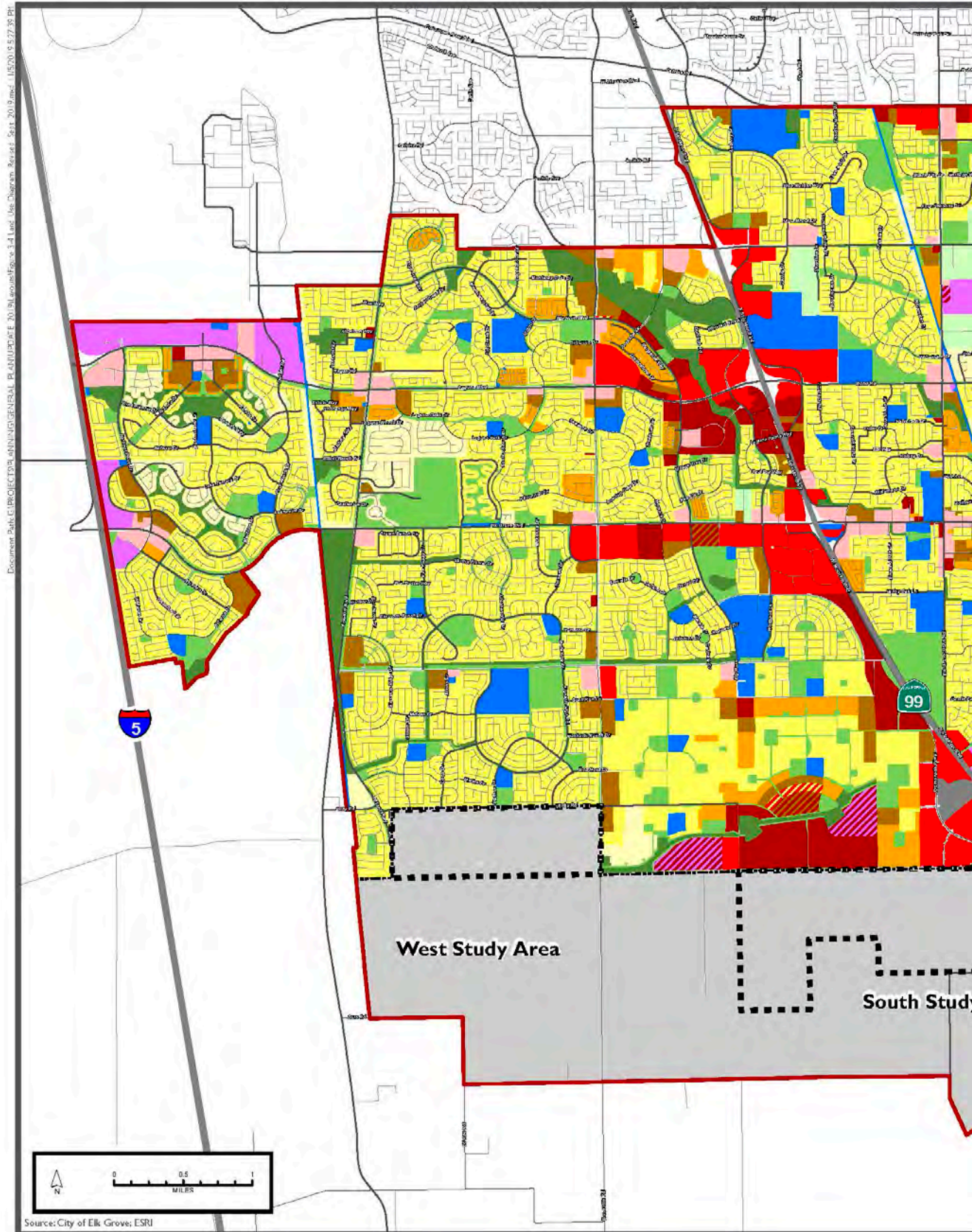
FIGURE 3-21 LAND USE
