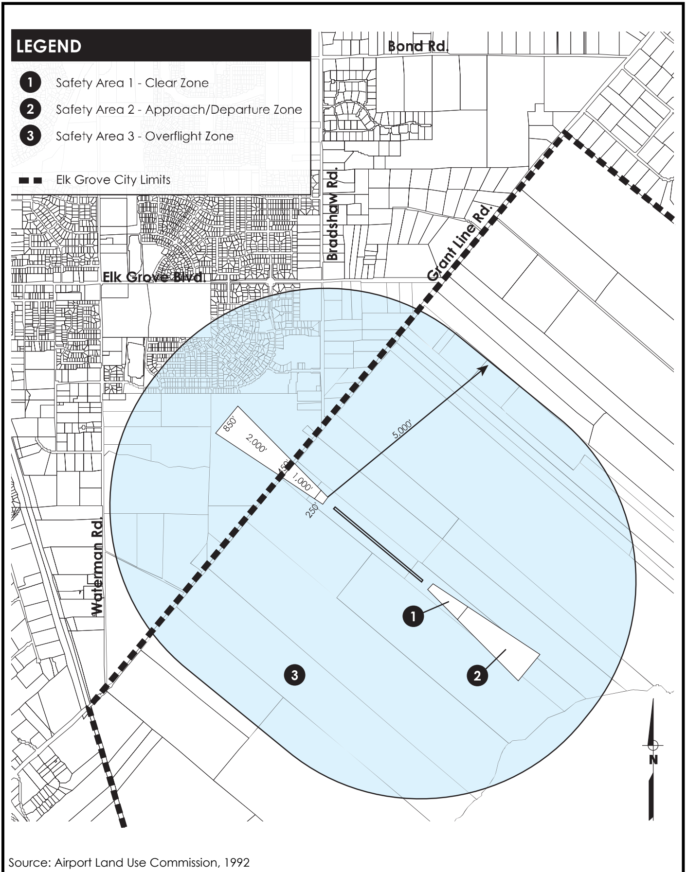
Figure 4.2-7 Clear, Approach/Departure and Overflight Zones - Sunset Skyranch Airport
