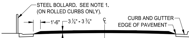
SPEED TABLE PLAN VIEW NOT TO SCALE
