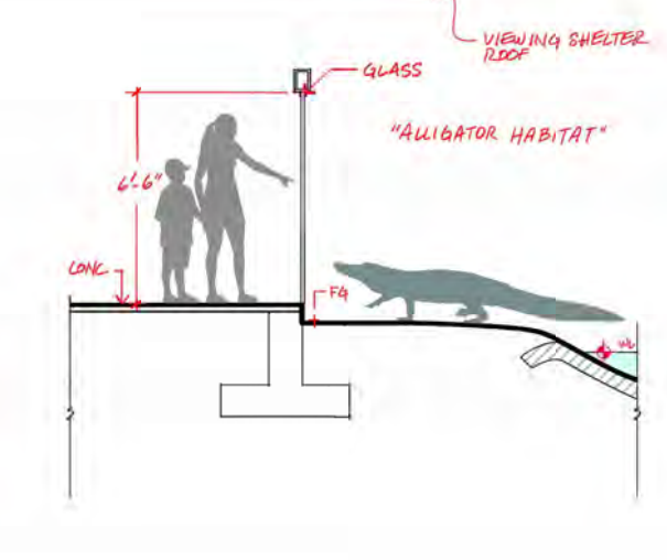
11 F4 - Alligator Glass Viewing - Section 1/2" = 1'-0"
