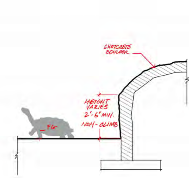
7 D3 - Tortoise Rockwork - Section 1/2" = 1'-0"
