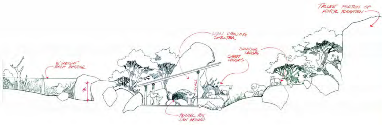
Entry to Lion Continued- Section 1/8" = 1'-0"
