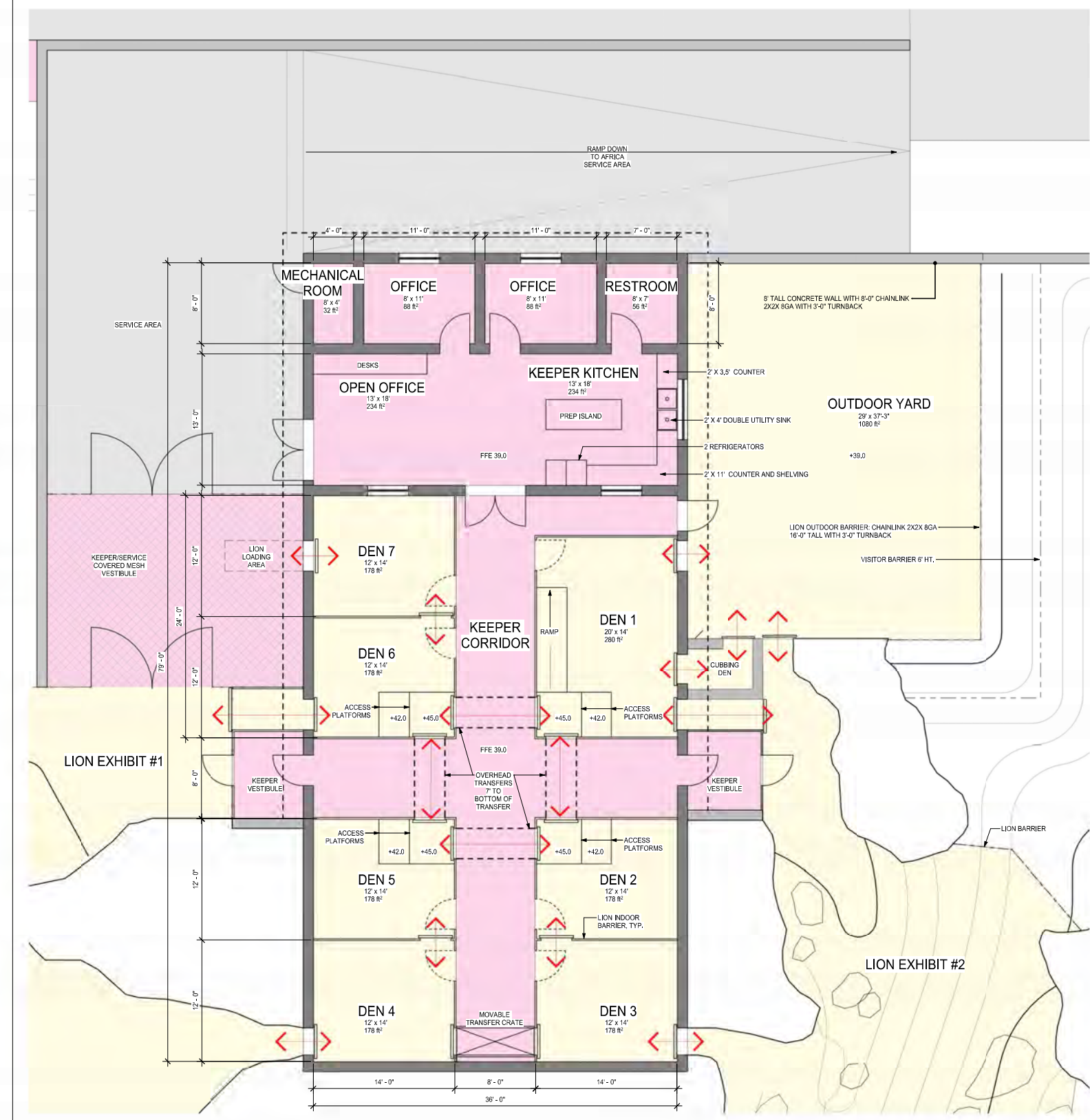
3 Lion Indoor Barrier NTS
