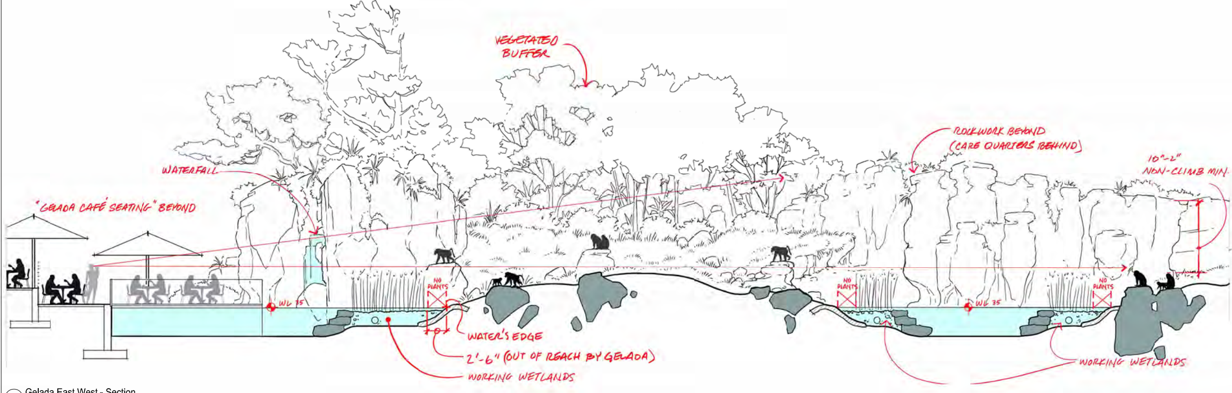
1 Gelada East West - Section 1/4" = 1'-0"
