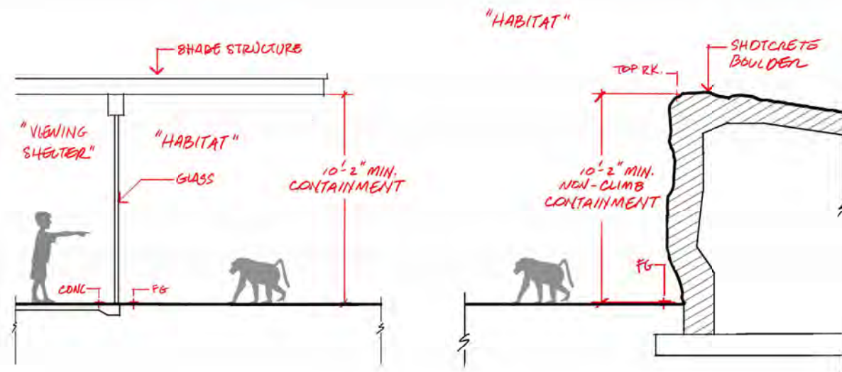
1 E1 - Gelada Glass Viewing - Section 1/2" = 1'-0"
