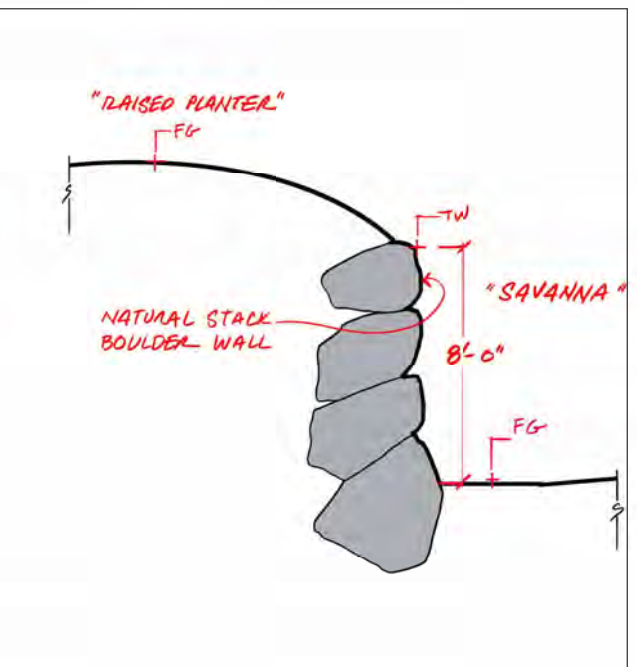
4 A4 & B4 Savanna Rock Wall - Section 1/2" = 1'-0"
