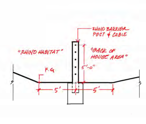
6 H3 - Rhino Cable - Section 1/2" = 1'-0"
