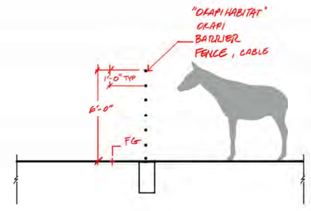
2 C2 - Okapi Fence - Section 1/2" = 1'-0"
