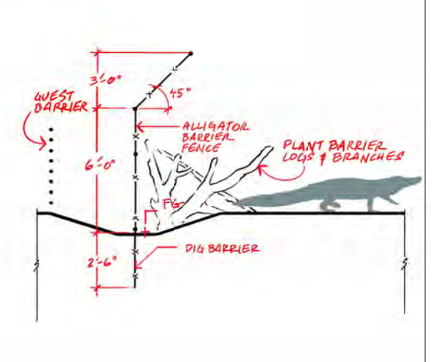
12 F5 - Alligator Fence - Section 1/2" = 1'-0"
