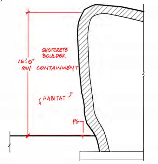
9 I2 - Lion Rockwork - Section 1/2" = 1'-0"
