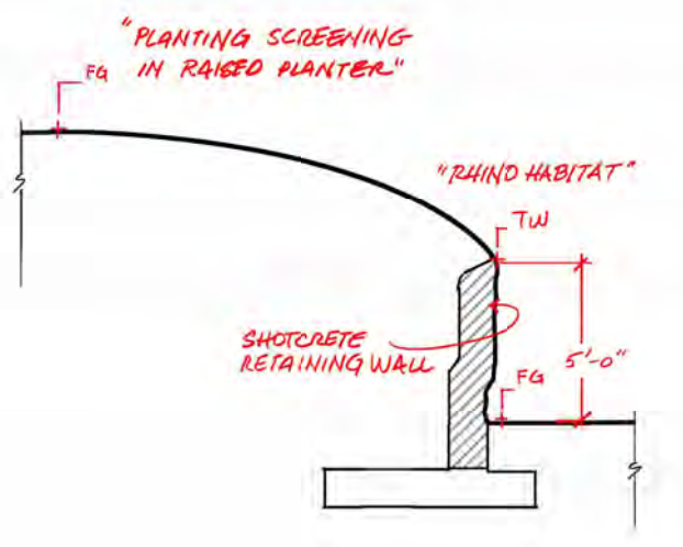
5 H2 - Rhino Mudbank - Section 1/2" = 1'-0"
