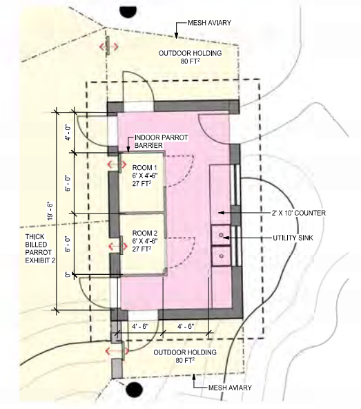
5 Parrot Care Quarters 1/4" = 1'-0"
