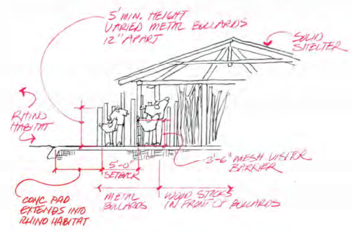
2 Rhino Boma - Section 1/4" = 1'-0"
