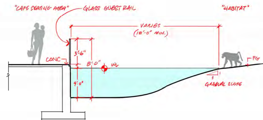
3 E3 - Gelada Water as a Barrier at Cafe - Section 1/2" = 1'-0"
