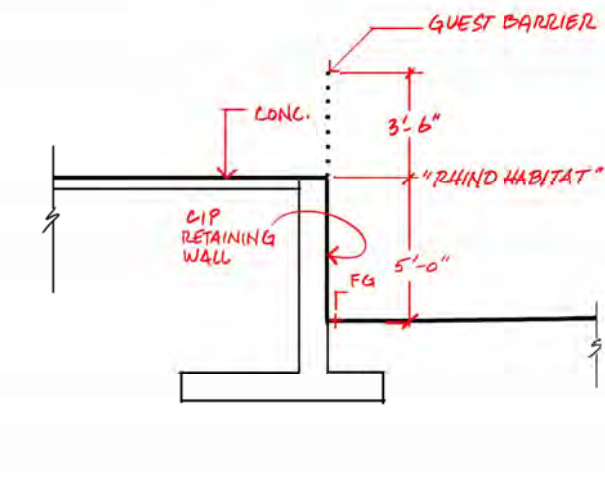
7 H4 - Rhino CIP Wall - Section 1/2" = 1'-0"
