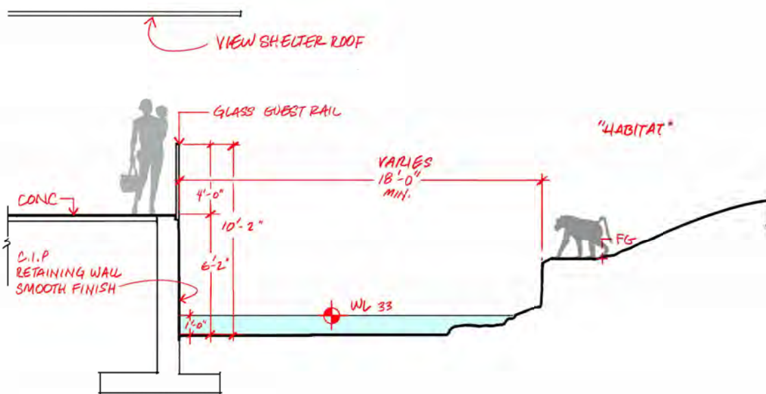
4 E4 - Gelada Retaining Wall and Fence - Section 1/2" = 1'-0"
