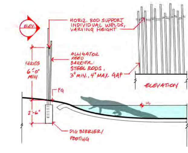
9 F2 - Alligator Reeds - Section 1/2" = 1'-0"
