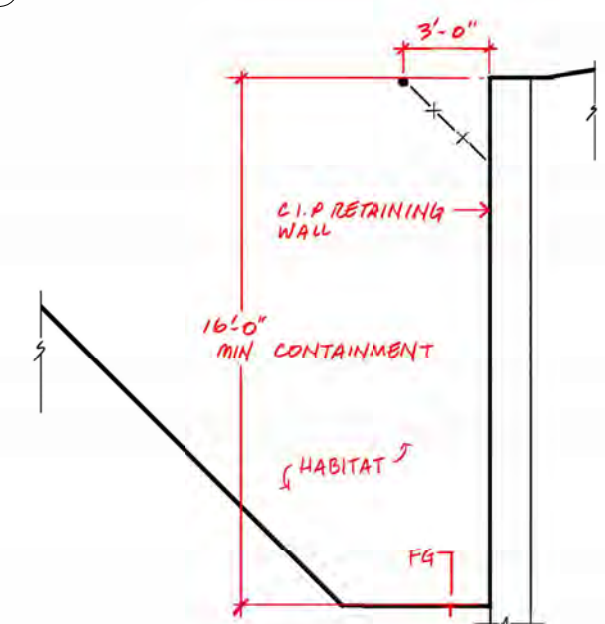
10 I3 - Lion CIP Wall - Section 1/2" = 1'-0"
