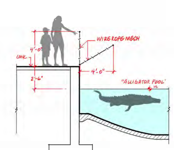
10 F3 - Alligator Glass Rail - Section 1/2" = 1'-0"
