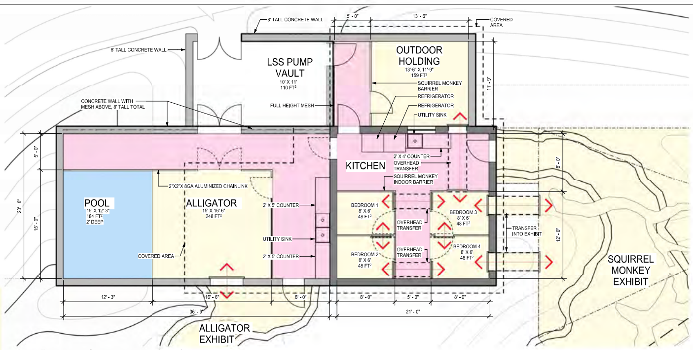
1 Alligator and Squirrel Monkey Care Quarters and Filtration 1/4" = 1'-0"
