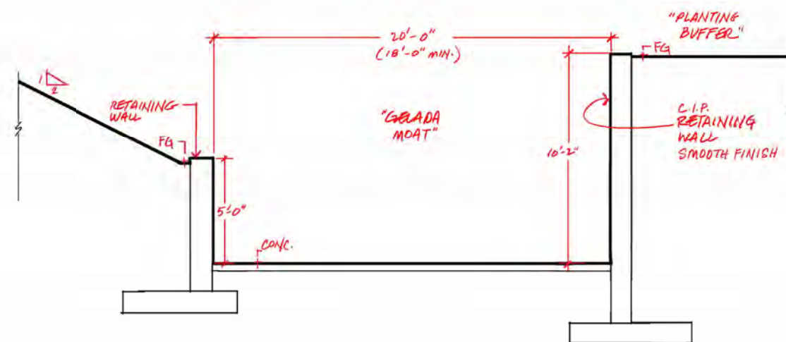
5 E5 - Gelada Retaining Moat Wall - Section 1/2" = 1'-0"
