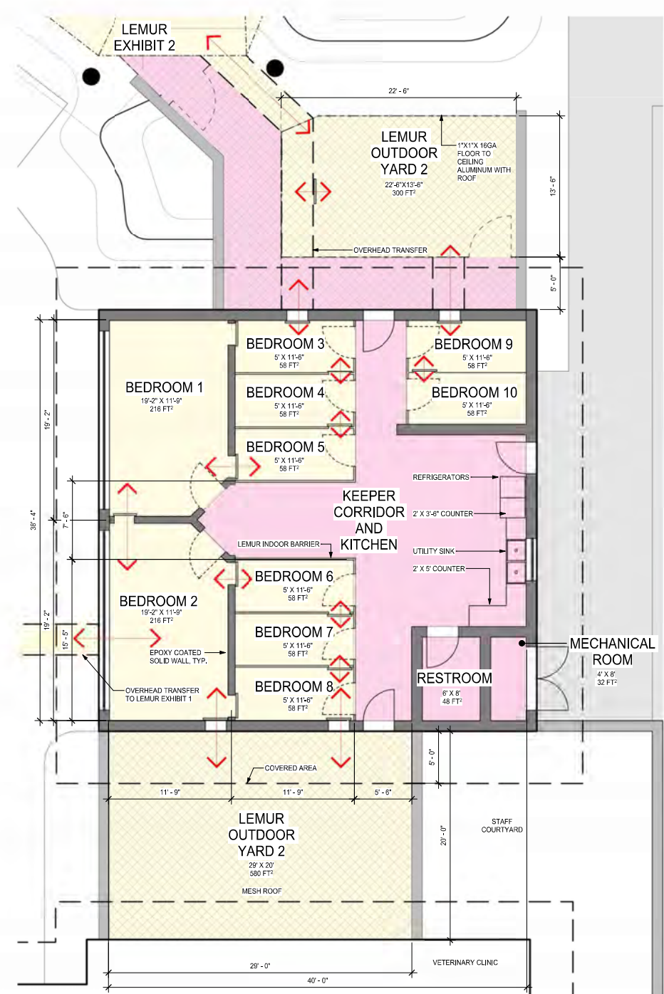
2 Lemur Care Quarters 1/4" = 1'-0"
