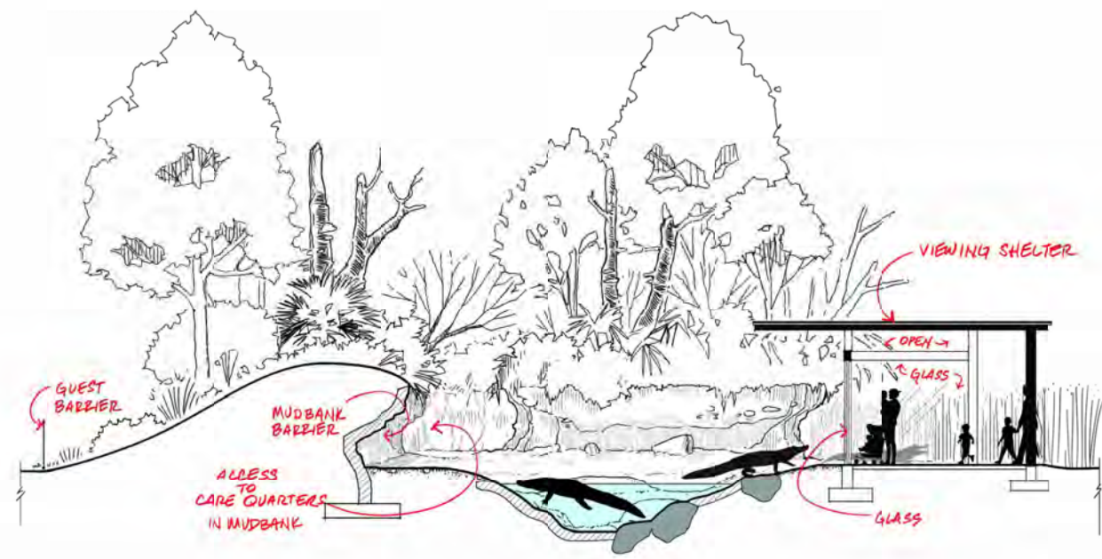
1 Alligator - Section 1/4" = 1'-0"
