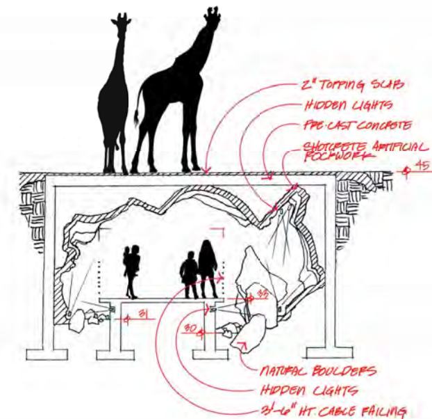
2 Savanna Tunnel - Section 1/4" = 1'-0"
