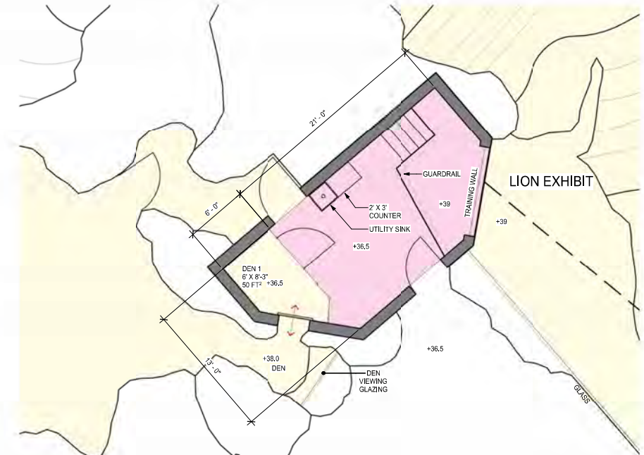
4 Lion Overhead Transfer 1" = 1'-0"
