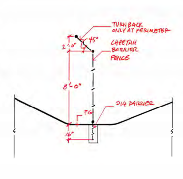
4 G4 - Cheetah Fence - Section 1/2" = 1'-0"
