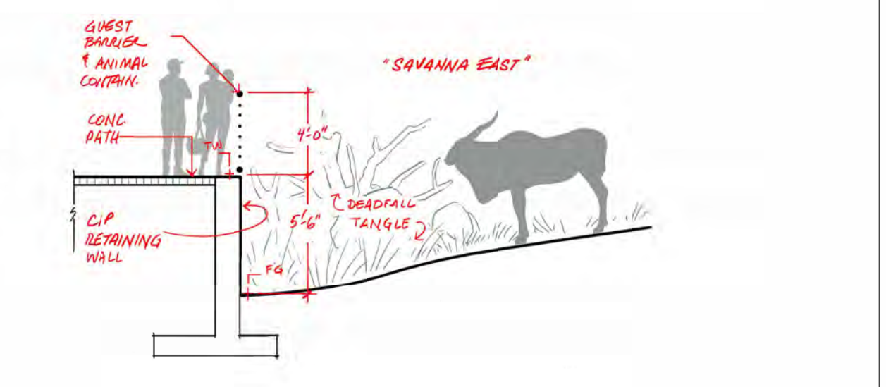
7 A5 Savanna CIP Wall View - Section 1/2" = 1'-0"
