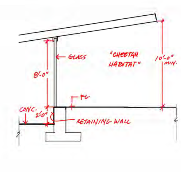
1 G1 - Cheetah Glass Viewing - Section 1/2" = 1'-0"
