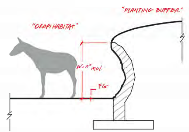
1 C1 - Okapi Mudbank - Section 1/2" = 1'-0"
