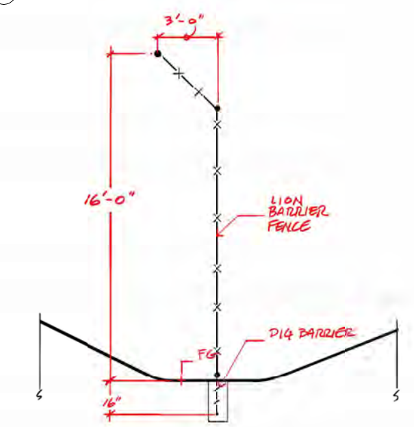
11 I4 - Lion Fence - Section 1/2" = 1'-0"
