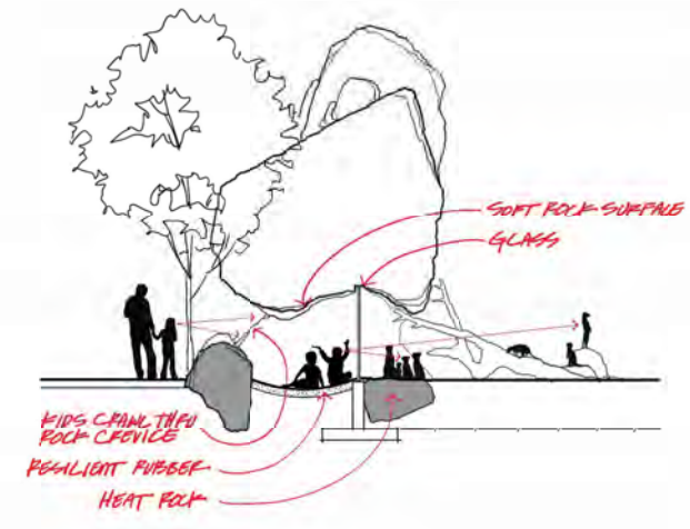
2 Meerkat Crawl-Through - Section 1/4" = 1'-0"
