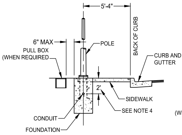
5' TO 6' SIDEWALK
