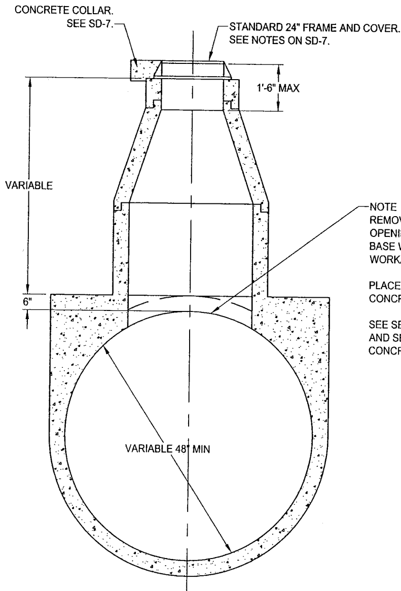
TYPE A CAST-IN-PLACE PIPE ONLY
